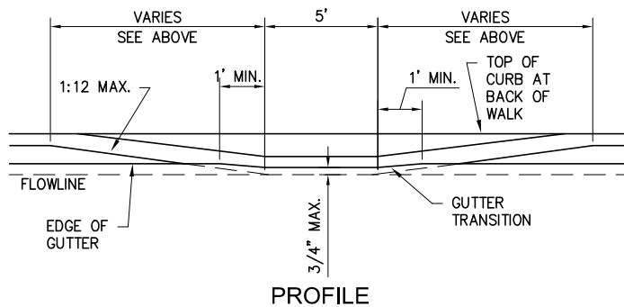
PAIRED RAMP IN CURB RETURN
