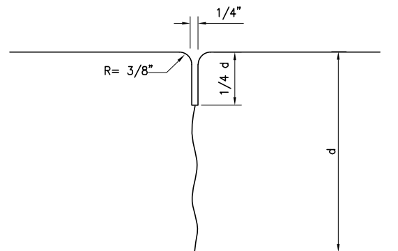
CONTROL JOINT
