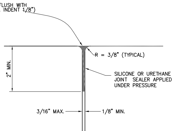
FORM PLATE JOINT
