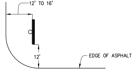
TYPICAL RURAL INSTALLATION
