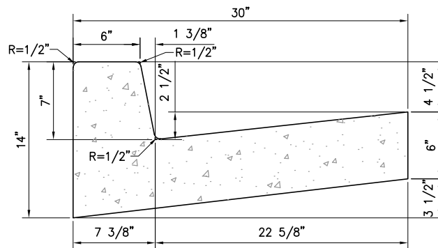
2.5' STANDARD CURB & GUTTER
