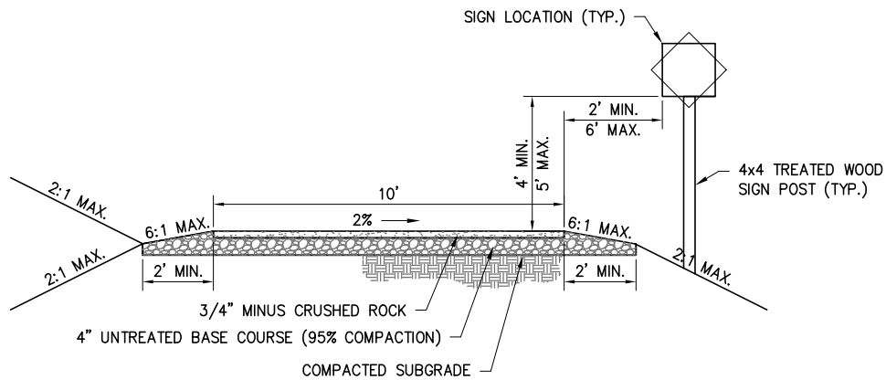
NATURAL TRAIL CROSS SECTION
