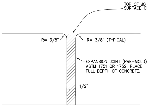
EXPANSION JOINT
