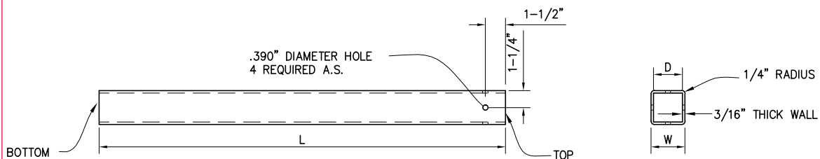
SIGN ANCHOR DETAIL
