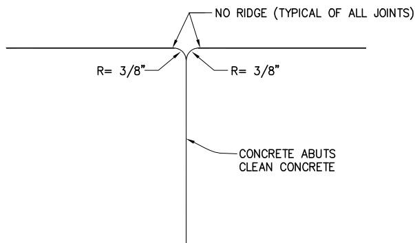
COLD JOINT
