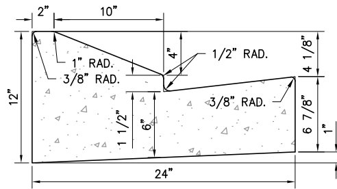
2.0' MODIFIED CURB & GUTTER
