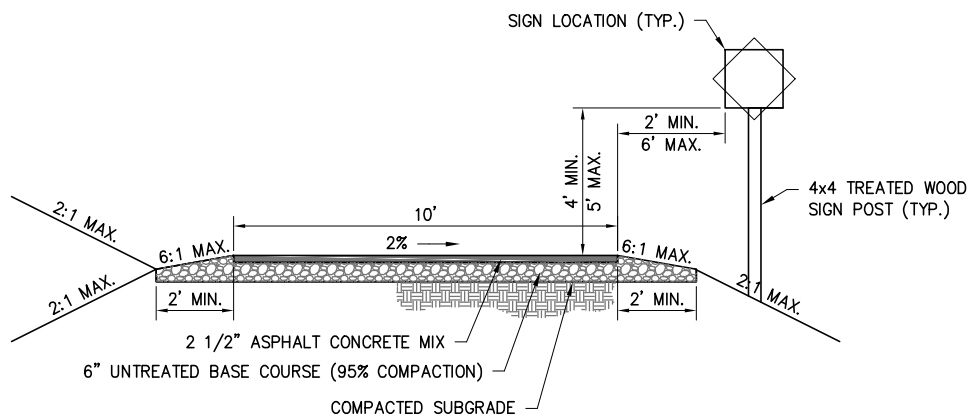
MULTI-USE TRAIL CROSS SECTION
