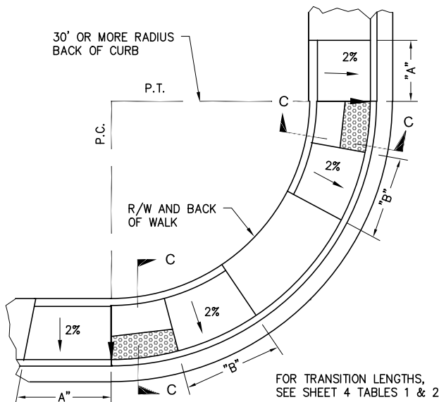
PAIRED RAMP IN CURB RETURN
