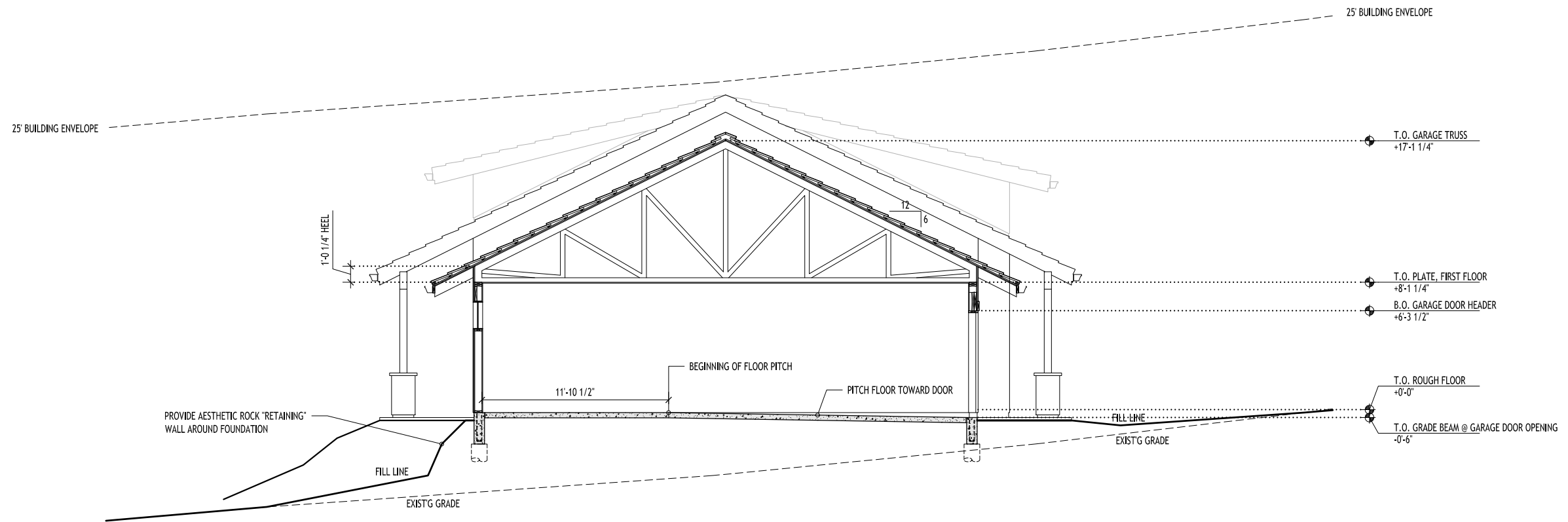
B-B Garage Cross Section
