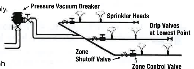
Multizone System
