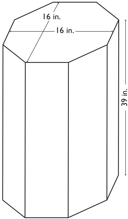
Octagonal Pedestal available for display (drawing not to scale)
